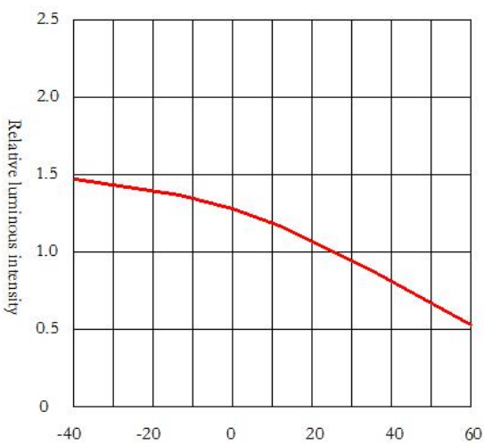
Ambient temperature Vs. Relative luminous intensity
