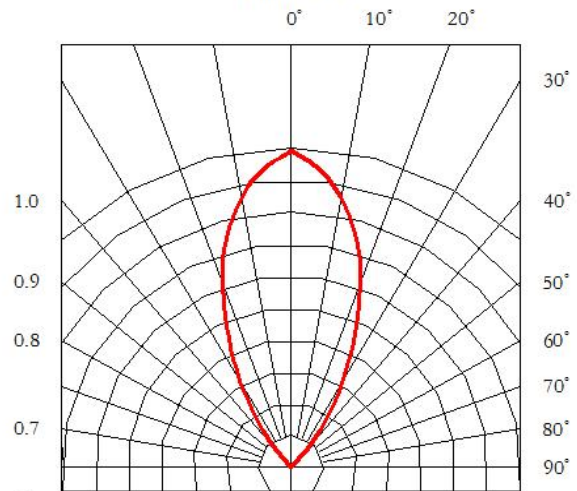
Radiation diagram
