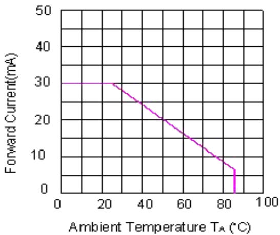
Forward Current Derating Curve, Derating based on T_{jMAX}=85^{\circ}\text{C}
