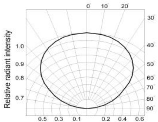
Fig.6 Radiation diagram
