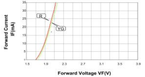
Fig.2 FORWARD CURRENT VS. FORWARD VOLTAGE
