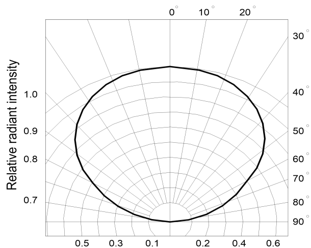
Fig.6 Radiation diagram
