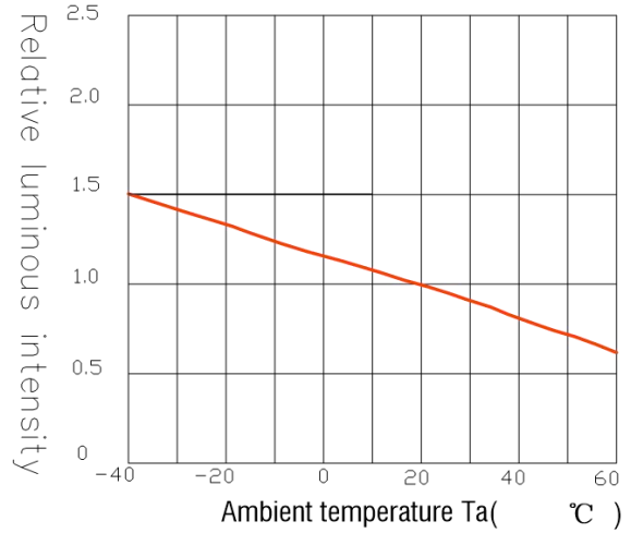
Fig.4 Relative luminous intensity Vs. Ambient temperature
